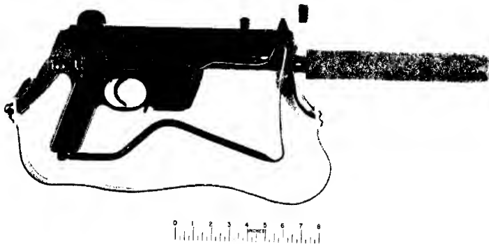
Figure 58. 9 mm MPK Walther Submachine Gun/West German Silencer
